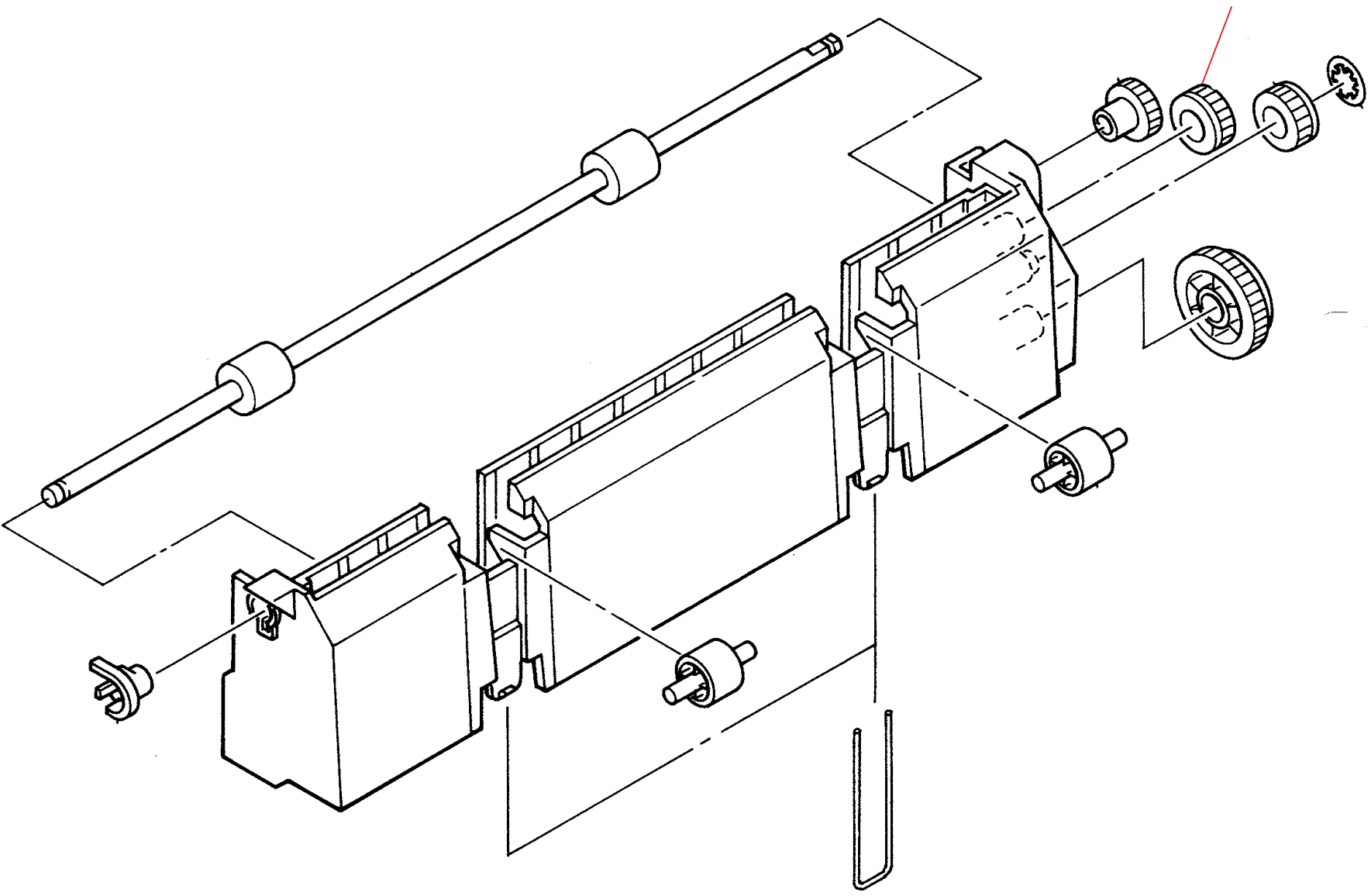
Fig.4 - Paper Path Adaptor (PA-20, for FS-1700/3700)
